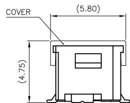
16~60 PIN - COVER
